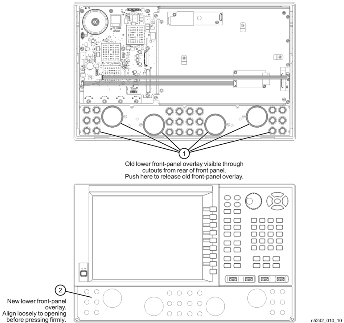
Figure 13 Lower Front Panel Overlay Replacement
