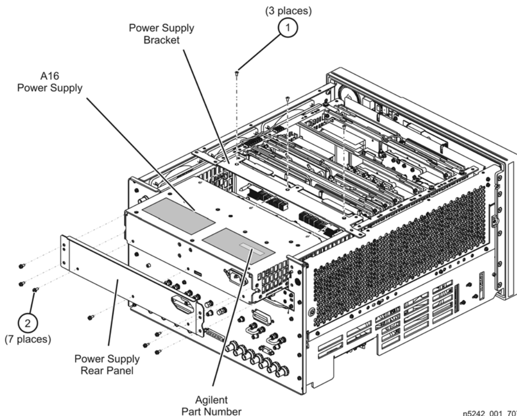
Figure 12 Power Supply Replacement
